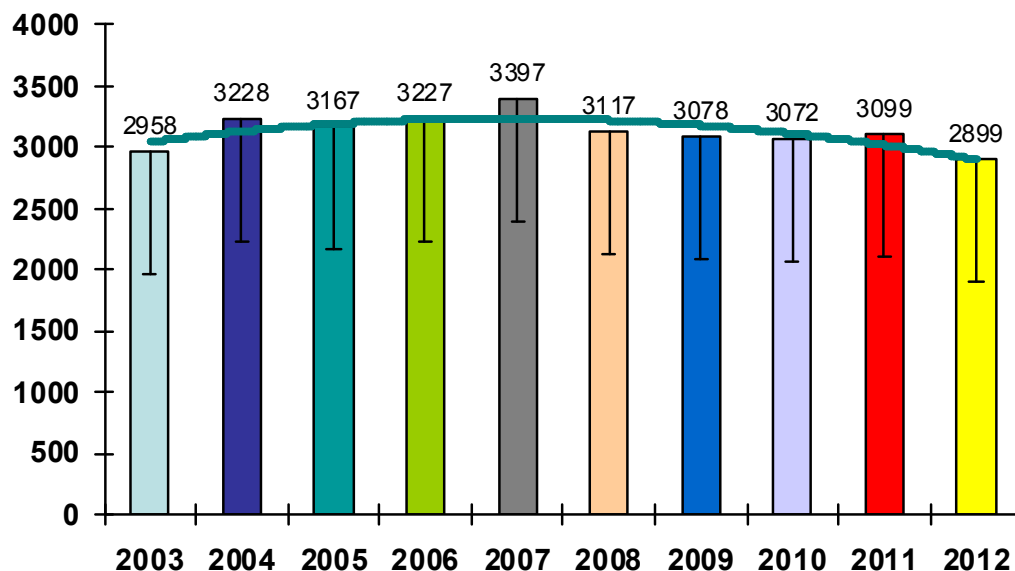
CHART-9.1 NUMBER OF ROAD ACCIDENTS (2003-2012)
