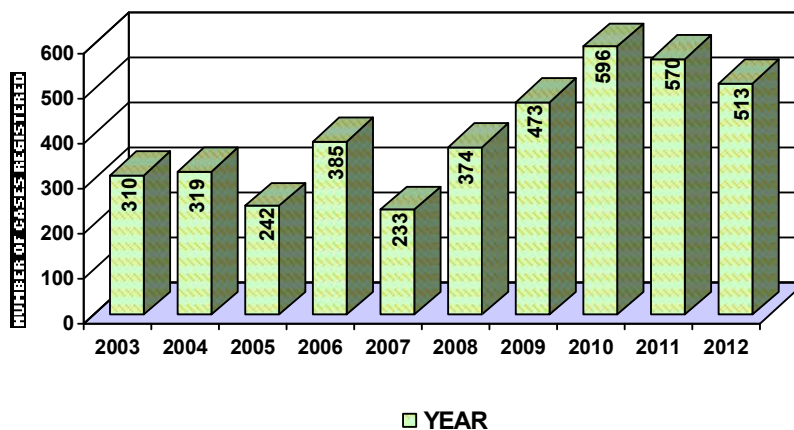
CHART-11.2 DETECTION UNDER ND&PS ACT DURING (2003-2012)
