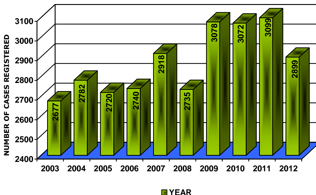
CHART-1.17 INCIDENCE OF ACCIDENTS DURING (2003-2012)
